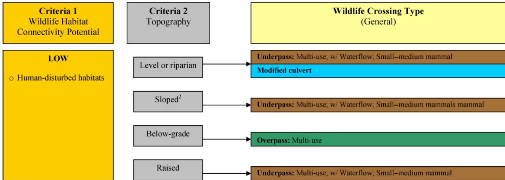
Figure 23. Chart. Criteria for selecting general wildlife crossing type where roads bisect habitats of low conservation value.
